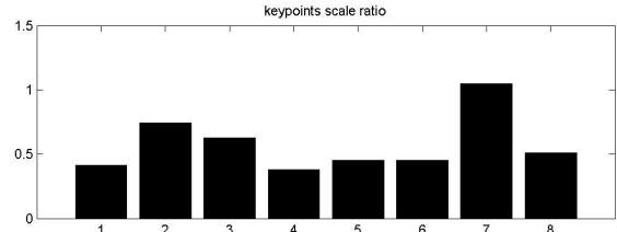
Figure 6: Correspondences between the two views and associated scale ratios of corresponding points. Note that the scale ratios of correspondences 2, 3 and 7 are noticeably above median value indicating inconsistent match.
