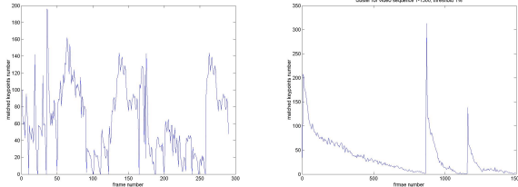
Figure 3: The number of keypoints matched between consecutive views for the sequence comprised of 18 locations (snapshot was taken every 2-3 meters) captured by a digital camera (left); the number of keypoints matched between the first and i -th view for a video sequence comprised of 3 locations (right).
