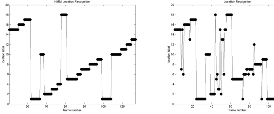
Seq. 2 with and without HMM
