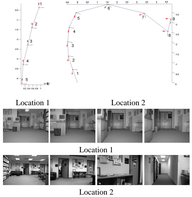
Figure 7: Relative positioning experiments with respect to the representative views. Bottom: Query views along the path between the first view and the representative view for two different locations. Top: Recovered motions for two locations.
